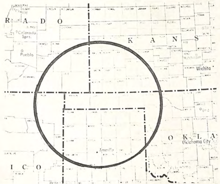
5 mv Groundwave Non-Directional
