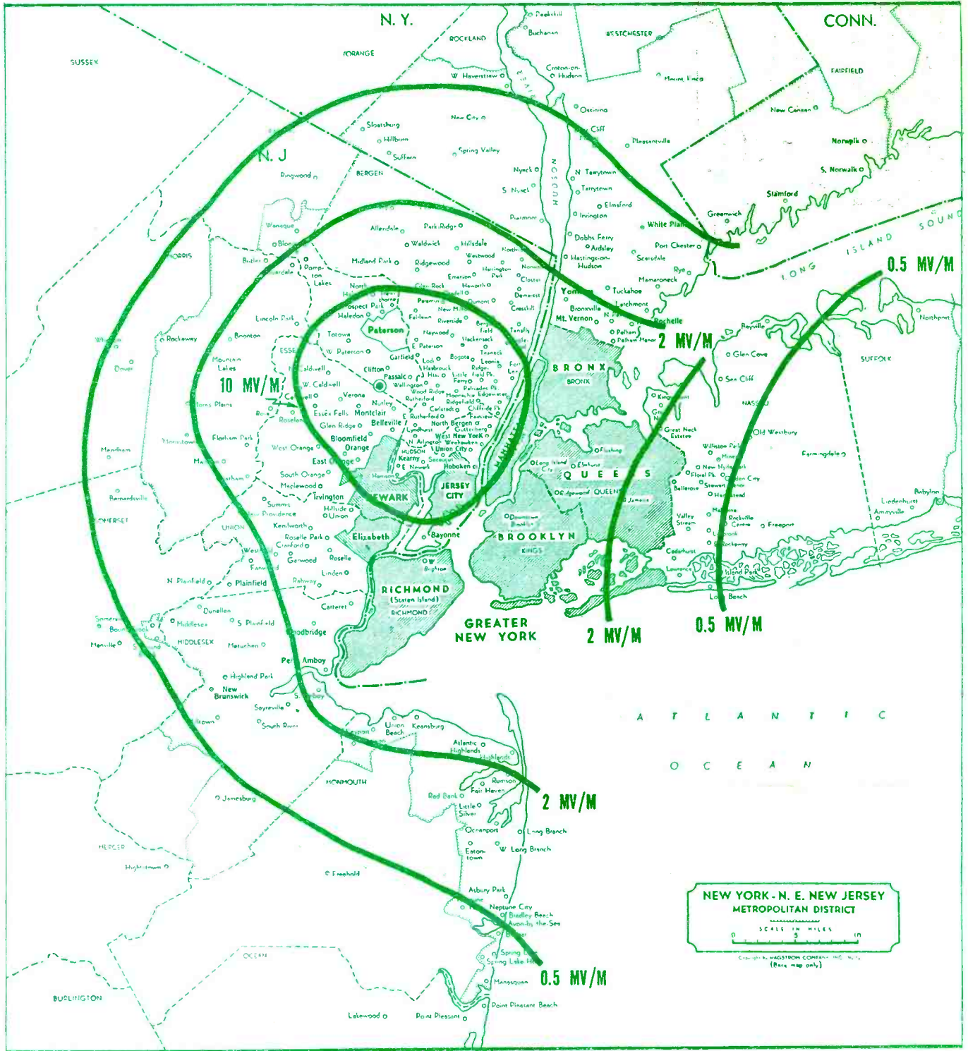
WPAT FIELD INTENSITY CONTOUR MAP
