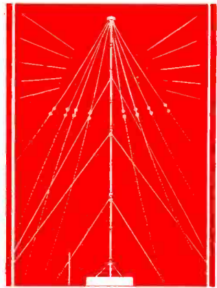
Diagram of the new high efficiency umbrella top loaded aerial system for maximum coverage strength.
