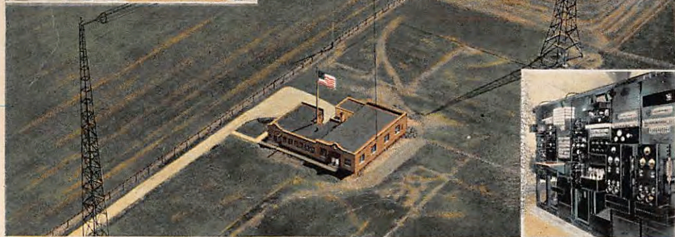
WTMJ'S TRANSMITTER WITH ANTENNAE TOWERS, AND BROADCASTING EQUIPMENT
